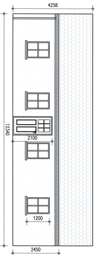
South Elevation 1:100
