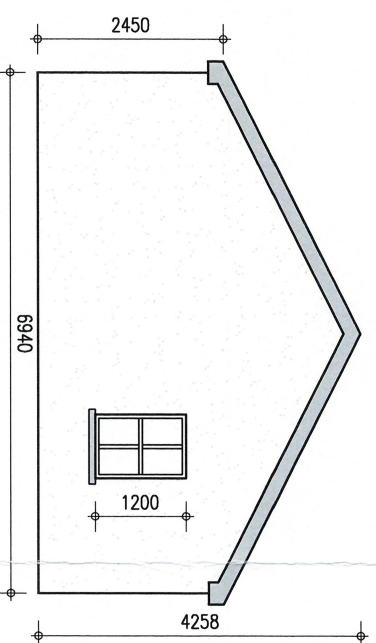
East Elevation 1:100
