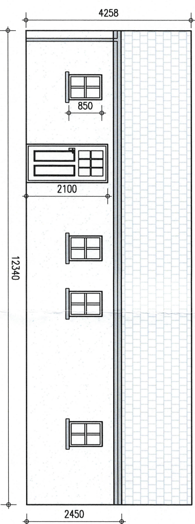
North Elevation 1:100
