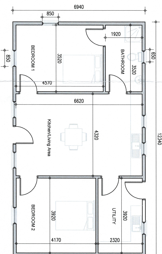
Floor Plans 1:100
